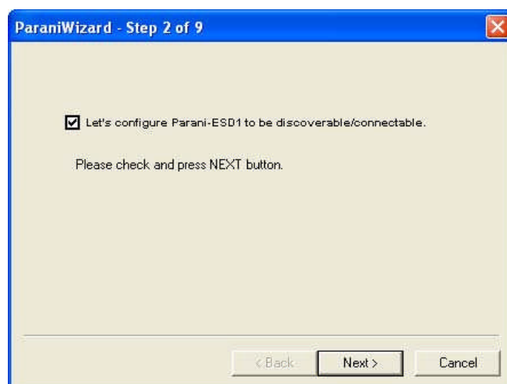
Figure 3-11 ParaniWizard Step 2
